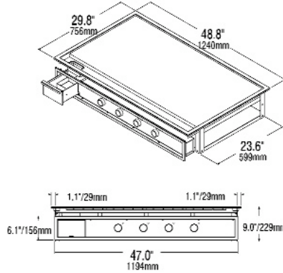
3D FRONT VIEW 148TDIG
