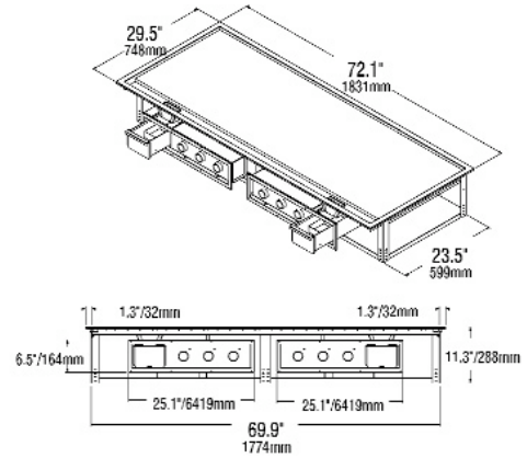
3D FRONT VIEW 172TDIG
